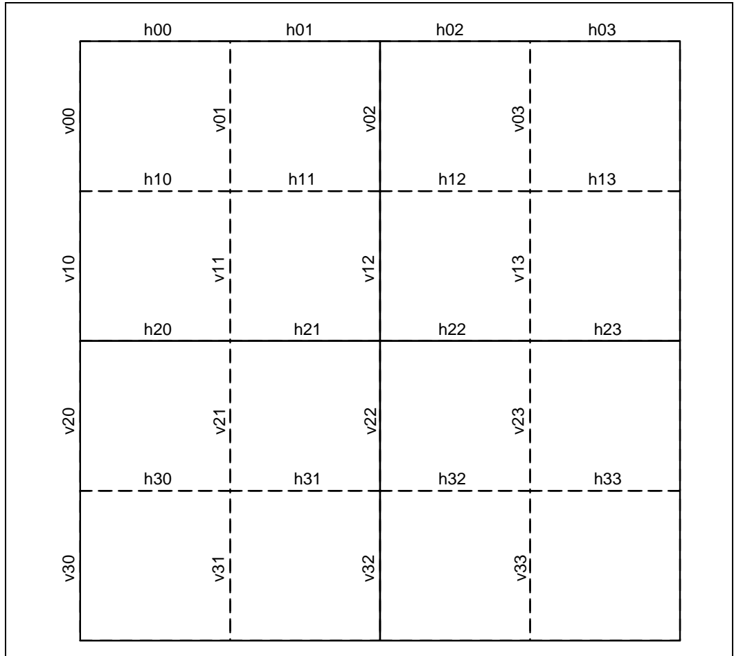
Figure 5-1. Boundary Values Layout in a Y Block
