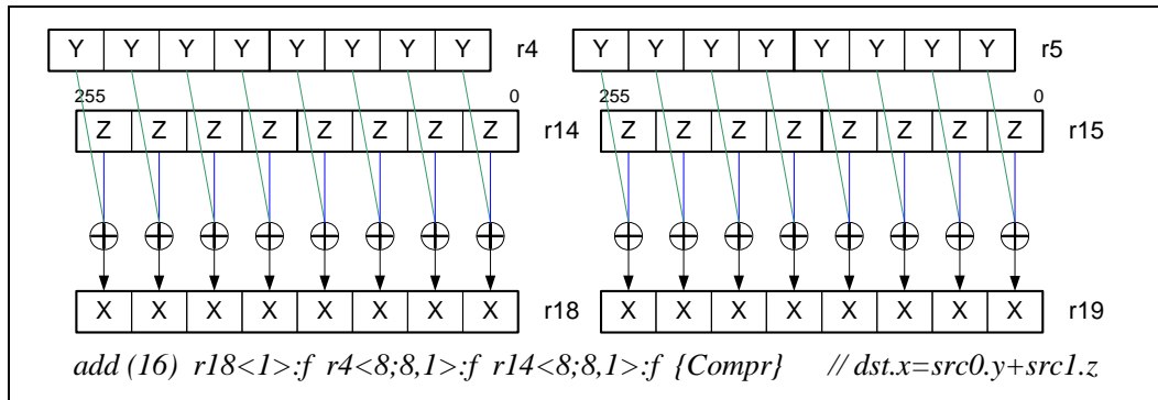
Figure 11-5. A SIMD16 Example
