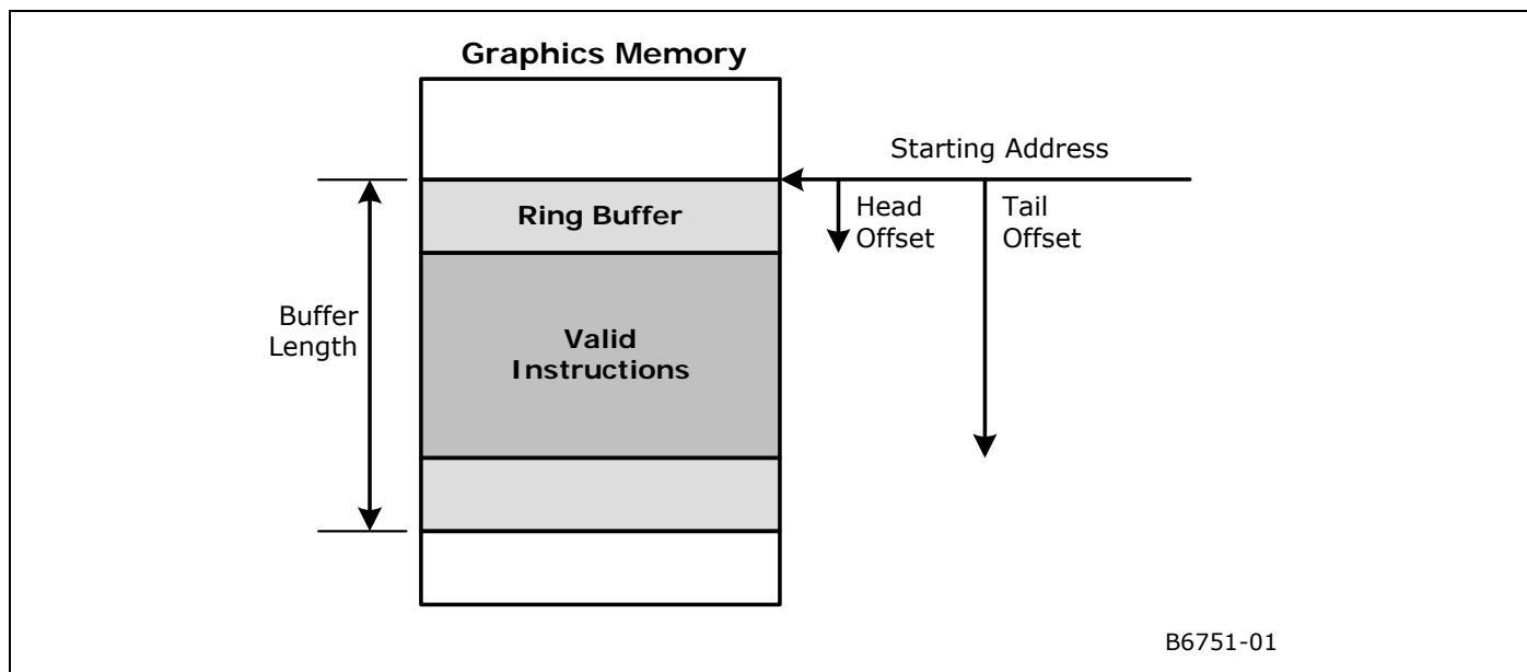
Figure 5-2. Ring Buffer
